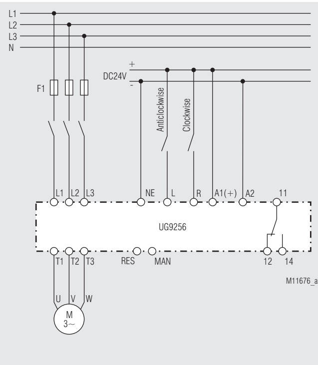
Motor control with UG 9256 and switch
