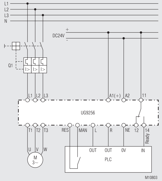
Motor control with UG 9256 and PLC
