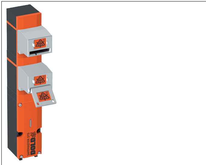
Presentation in the activated state: 1st key inserted; 2nd key removed
