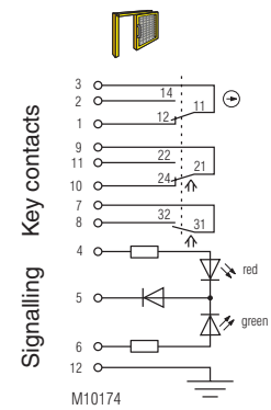
Fig. 2: Lock deactivated: 1st key inserted (bottom) 2nd key removed (top)
